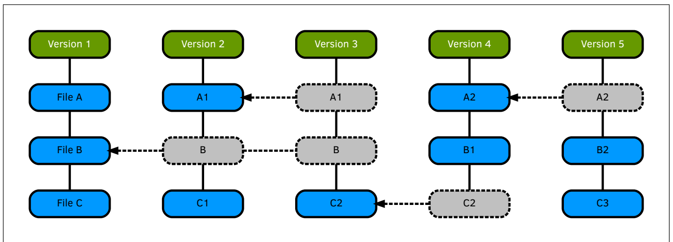
Figure 2. Git snapshots / file storage model
